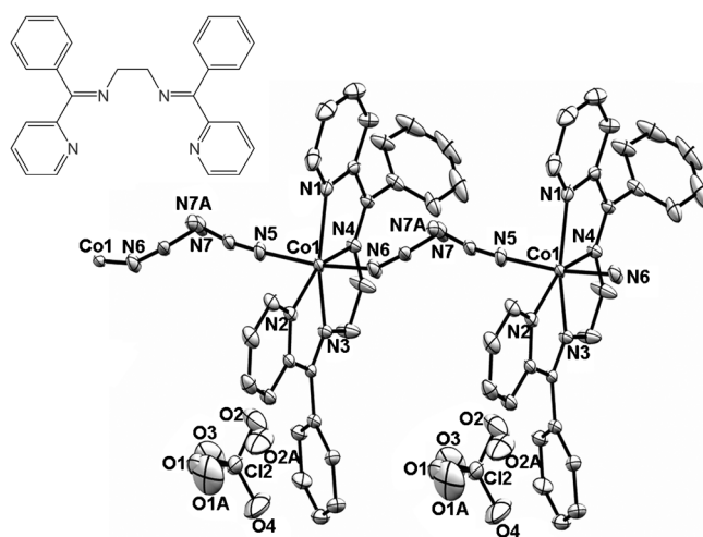
Figure 1. An ORTEP representation of a segment of the 1D chain along the b axis in 1 RT with HS Co II . Ellipsoids set at 30% probability; hydrogen atoms omitted for clarity. Inset: The enbpy ligand.
