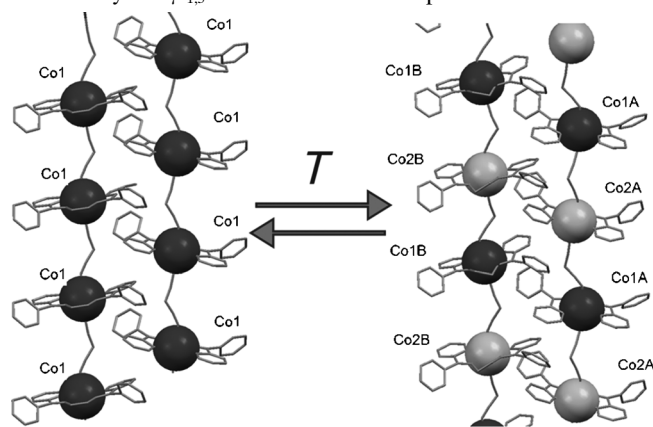
Figure 4. View of the 1D chains evolution during the SCO process along the c axis. HS Co dark gray, LS light gray.
