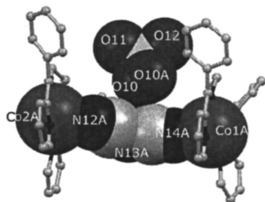
Figure 5. The supramolecular anion– \pi interaction in 1 LT involving O10 of the disordered perchlorate unit and the \pi cloud of a dicyanamide bridge ( \text{N12A}\cdots\text{C55A}\cdots\text{N13A}\cdots\text{C56A}\cdots\text{N14A} ).
